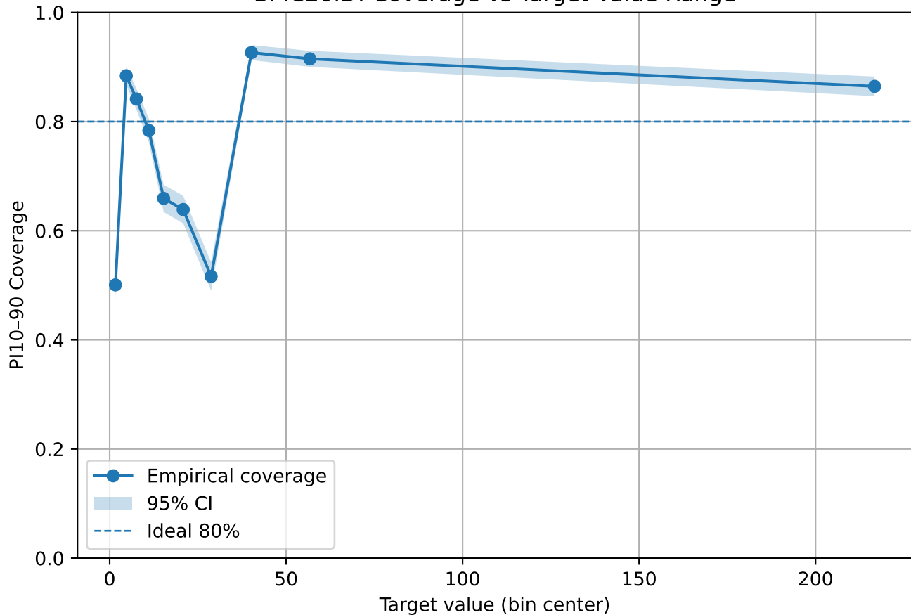
BPIC201D: Coverage vs Target Value Range
